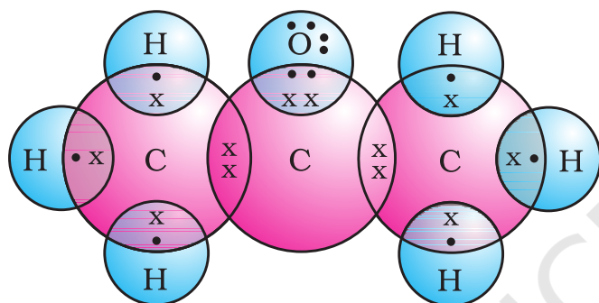
Electron dot structure of propanone
