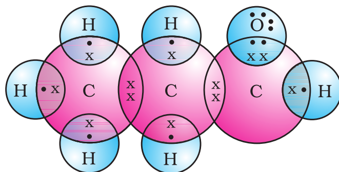
Electron dot structure of propanal
